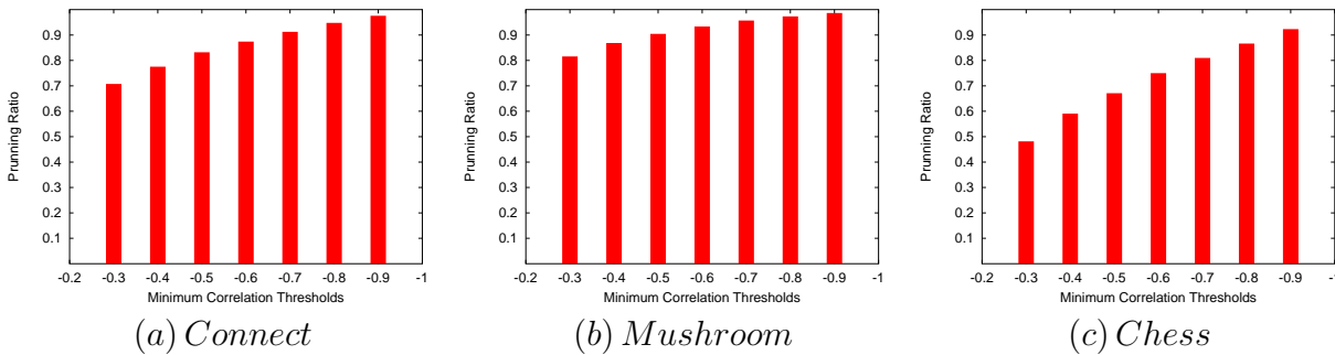
Fig. 21. The pruning effect for negative correlation computation on UCI Connect , Mushroom , Chess data sets.
