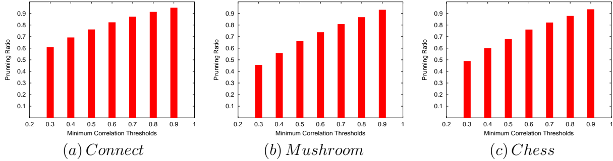
Fig. 14. The pruning effect of TAPER on UCI Connect , Mushroom , Chess data sets.
