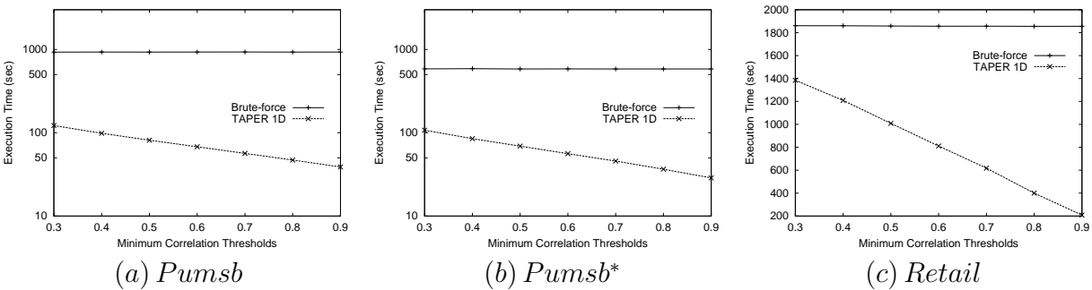
Fig. 12. TAPER 1D vs. a brute-force approach on the Pumsb , Pumsb* , and retail data sets.
