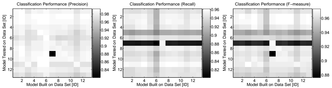
Figure 6: Generalizability of the scheme. The performance of different model on different data sets in terms of precision, recall and F-measure (from left to right)
